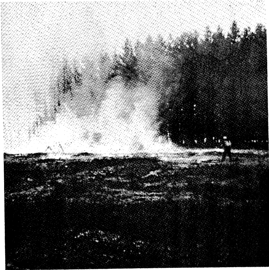
FIG. 3. Fire C6 following collapse after the wind failed. Note surface fire inside stand moving from left to right.
